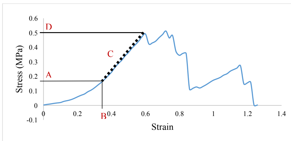
Figure 13. Stress-strain curve of a single layer tensile test indicating variables of interest: A) stress at the end of the toe region, B) strain at the end of the toe region, C) Young's modulus (slope of linear region), and D) yield point.
